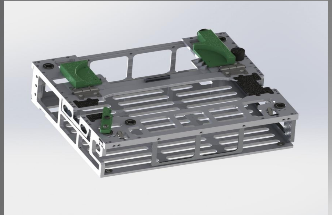
Workpiece carrier
