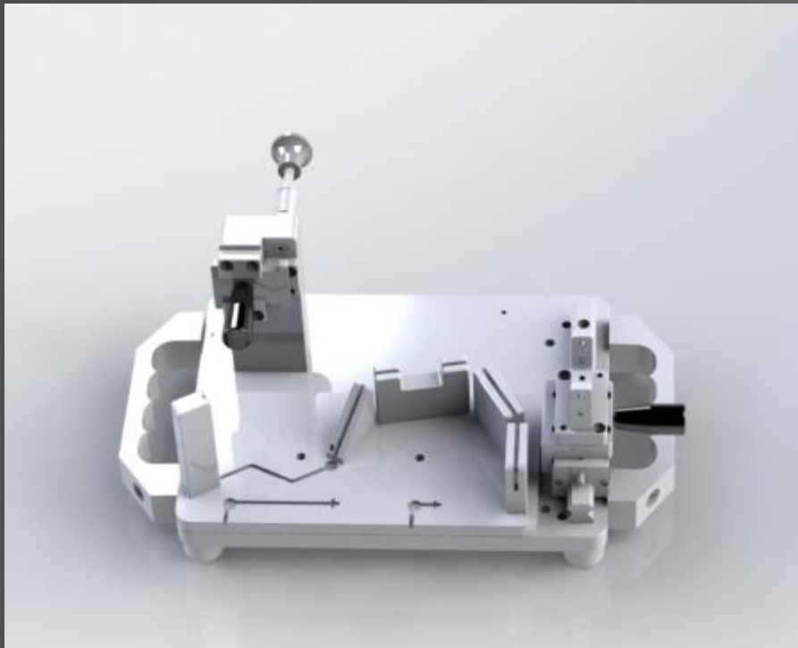
Finished product inspection and leveling device
