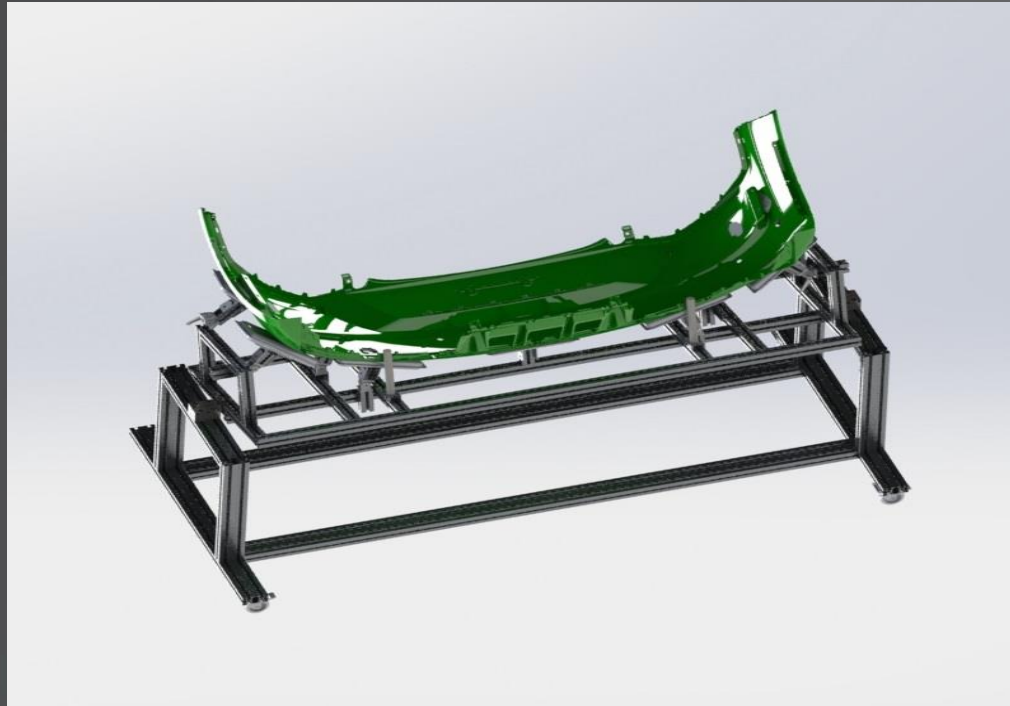
Workpiece carrier
